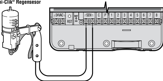
Mini-Clik® Regensensor
