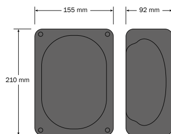
Multibox: S 60/100 • RC Dim 60/100 RC RGB • DALI • DMX
